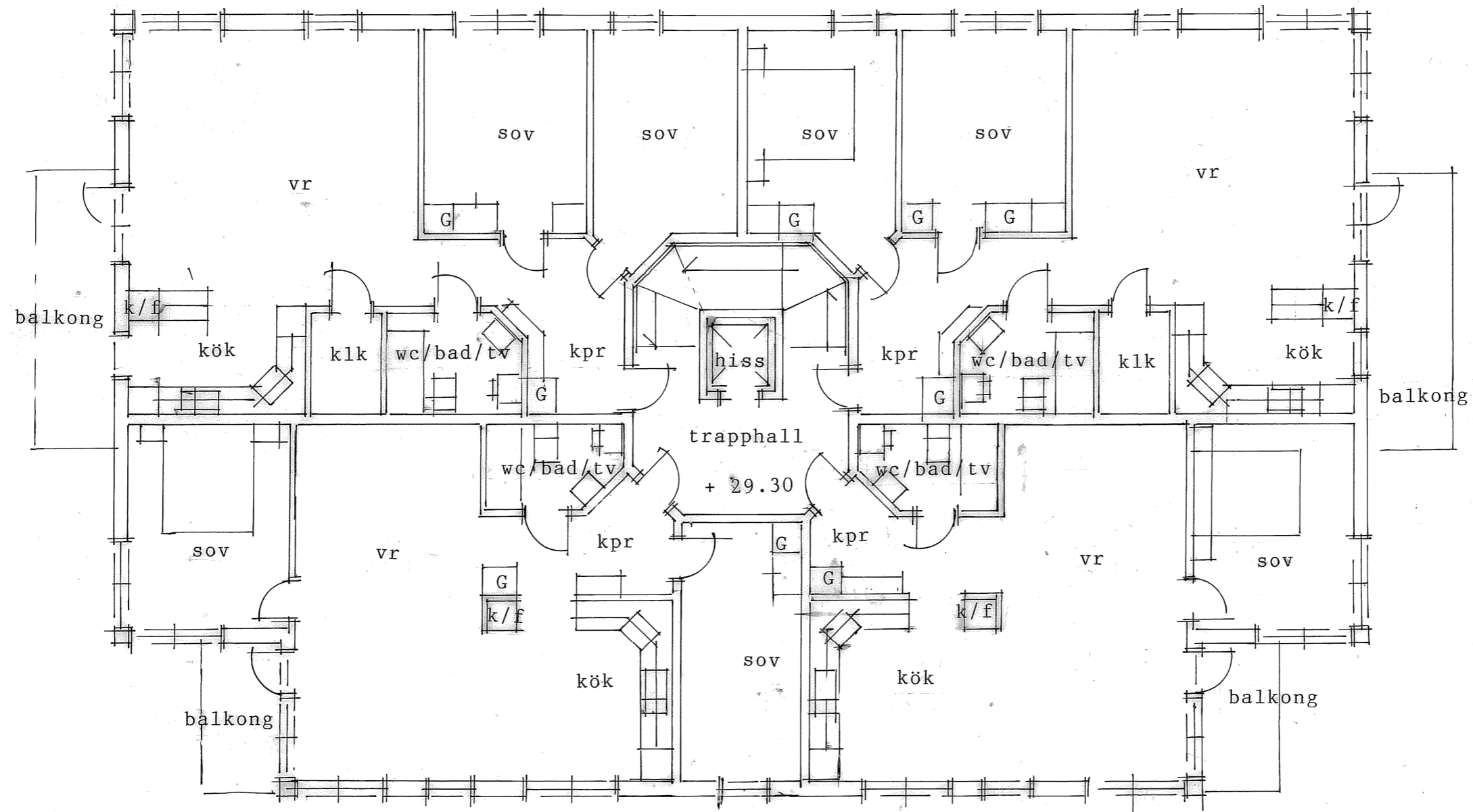
PLAN 1 tr
